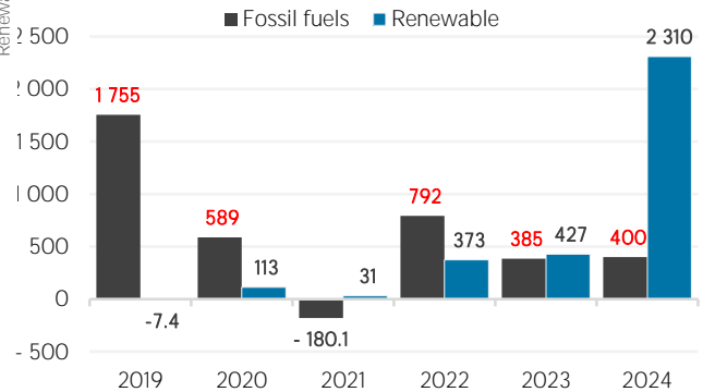
Net capacity change in 2024 (MW)
